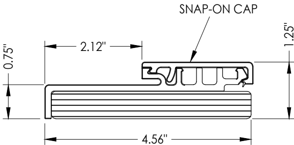
2 SIDE JAMB (2-PIECE)
