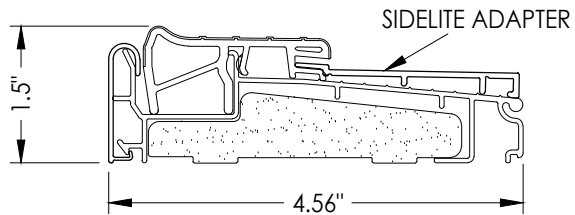
23 OUTSWING THRESHOLD w/ SIDELITE ADAPTER ENDURA
